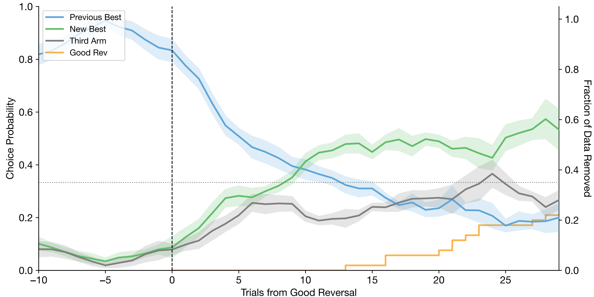
Good Reversal-Aligned Choices (mean \pm se across subjects | n=6 subjects, n=50 reversals)
